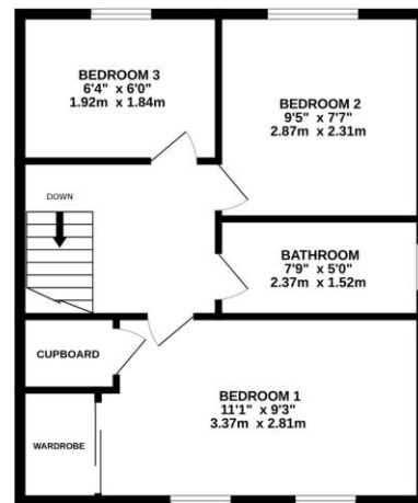
1ST FLOOR 581 sq.ft. (53.9 sq.m.) approx.
