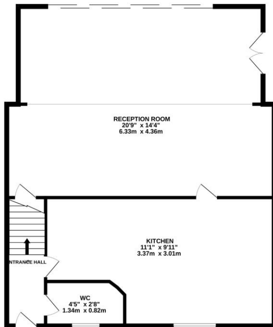
GROUND FLOOR 1189 sq.ft. (110.5 sq.m.) approx.
